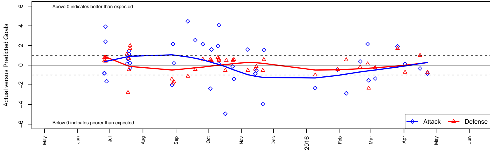
Washington Timbers Red B01 Dots are actual minus expected GF (blue circles) and GA (red triangles). Blue line is smoothed change in attack strength. Red is smoothed change in defense strength.
